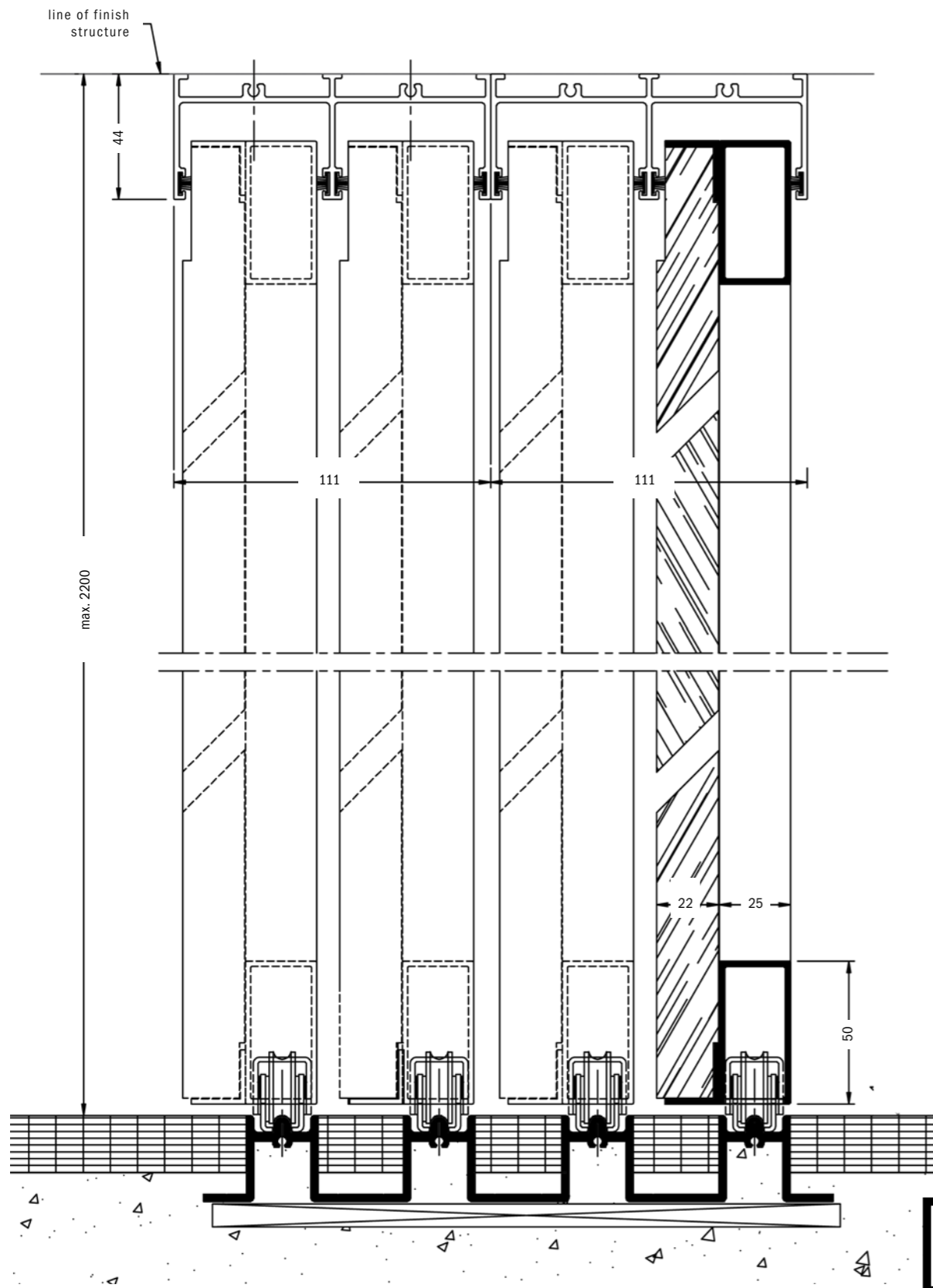
TIMBER SLAT SLIDING SHUTTER DETAIL (4 leaf shutter)
